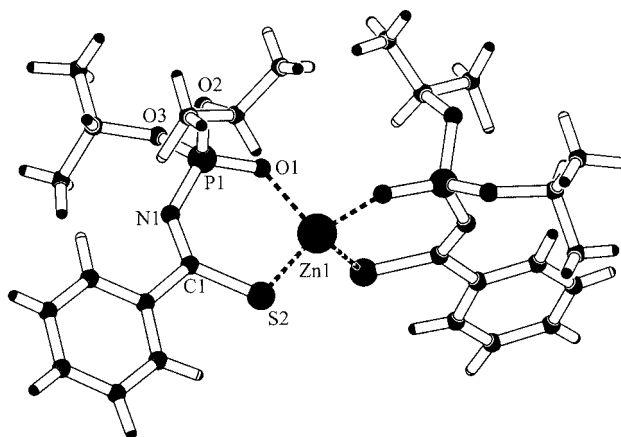
Figure 3. Molecular structure of complex 1 .
