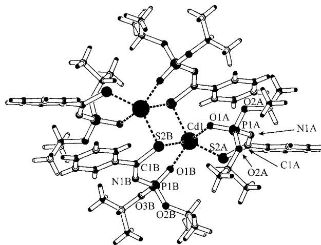
Figure 4. Molecular structure of complex 2 .
