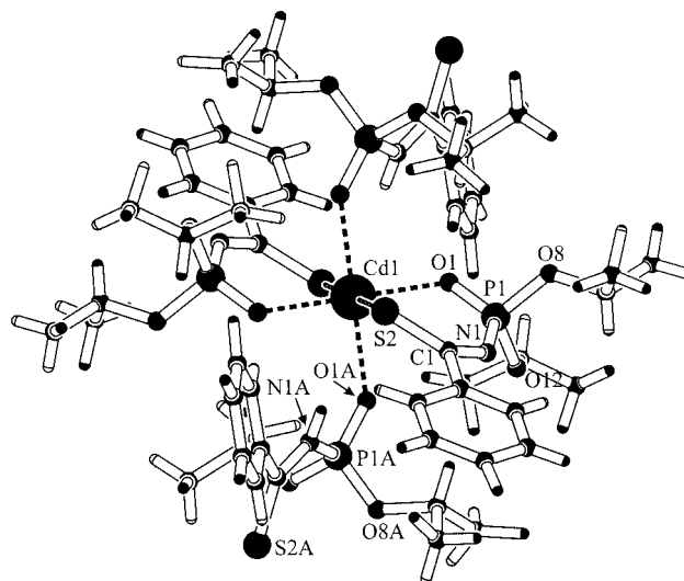
Figure 5. Molecular structure of complex 3 .
