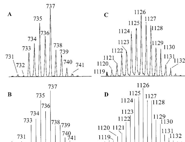
Figure 2. ES-MS spectra of complex 2 . Peak A is observed for the [CdL 2 + Na] + cation, pattern B is calculated for C 26 H 38 CdN 2 NaO 6 P 2 S 2 , peak C is observed for the [Cd 2 L 3 ] + cation and pattern D is calculated for C 39 H 57 Cd 2 N 3 O 9 P 3 S 3 .
