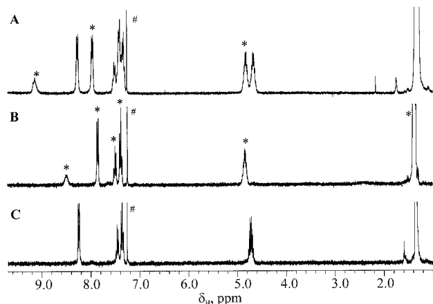
Figure 1. 1 H NMR spectra of complexes 3 (A), 2 (C) and HL (B). Signals of HL (free and in the structure of 3 ) are marked * and a signal for the solvent #.
